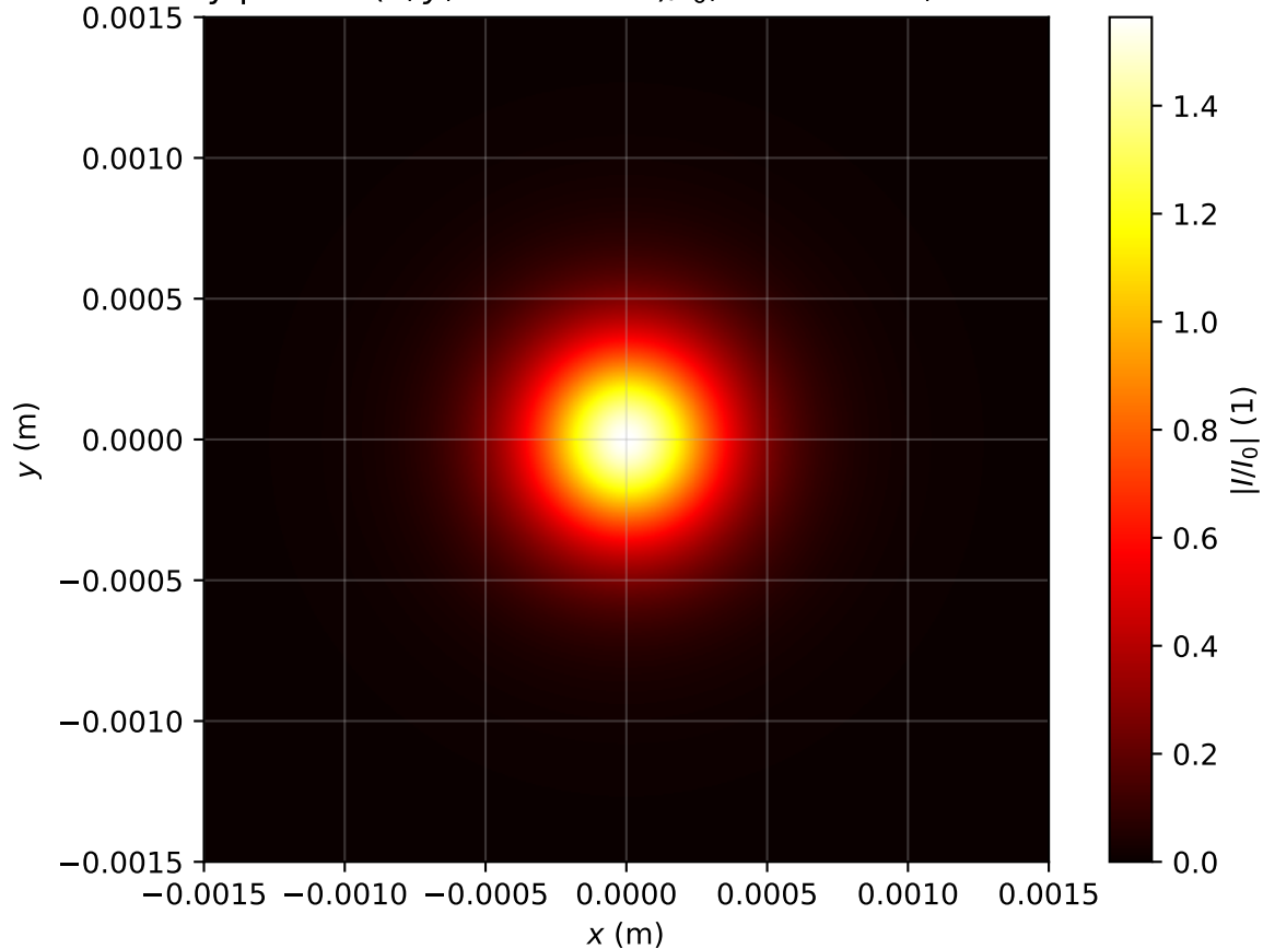
Intensity profile I(x, y, z = 3.025m)/I_0 , Pin=0.9Pcr, artificial time
